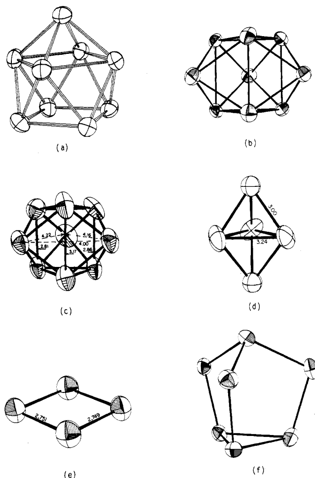
Figure 2. Some homopolyatomic Zintl anion structures established by X-ray crystallography: (a) \text{Sn}_9^{4-} , (b) \text{Sn}_9^{3-} , (c) \text{Ge}_9^{2-} , (d) \text{Pb}_5^{2-} , (e) \text{Bi}_4^{2-} , (f) \text{Sb}_7^{3-} (50% probability thermal ellipsoids; references in Table II).
