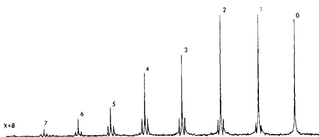
Figure 5. The 18.7-MHz ^{207}\text{Pb} power spectrum (increasing field) for a mixture of \text{Sn}_x\text{Pb}_{9-x}^{4-} ions in en ( \text{Rb}^+ cations; J(^{207}\text{Pb}-\text{Sn}) \approx 540 – 473 Hz). Reproduced with permission from ref 75. Copyright University of Michigan, 1982.
